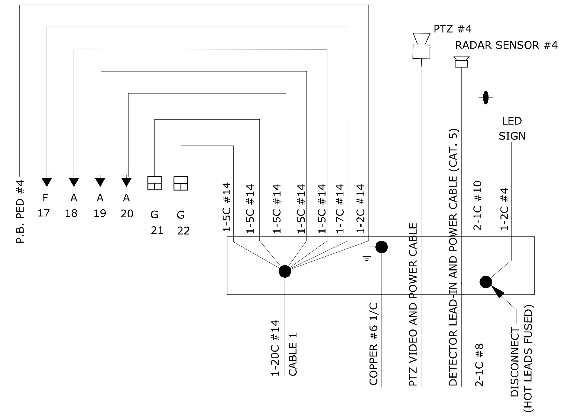
POLE #4
