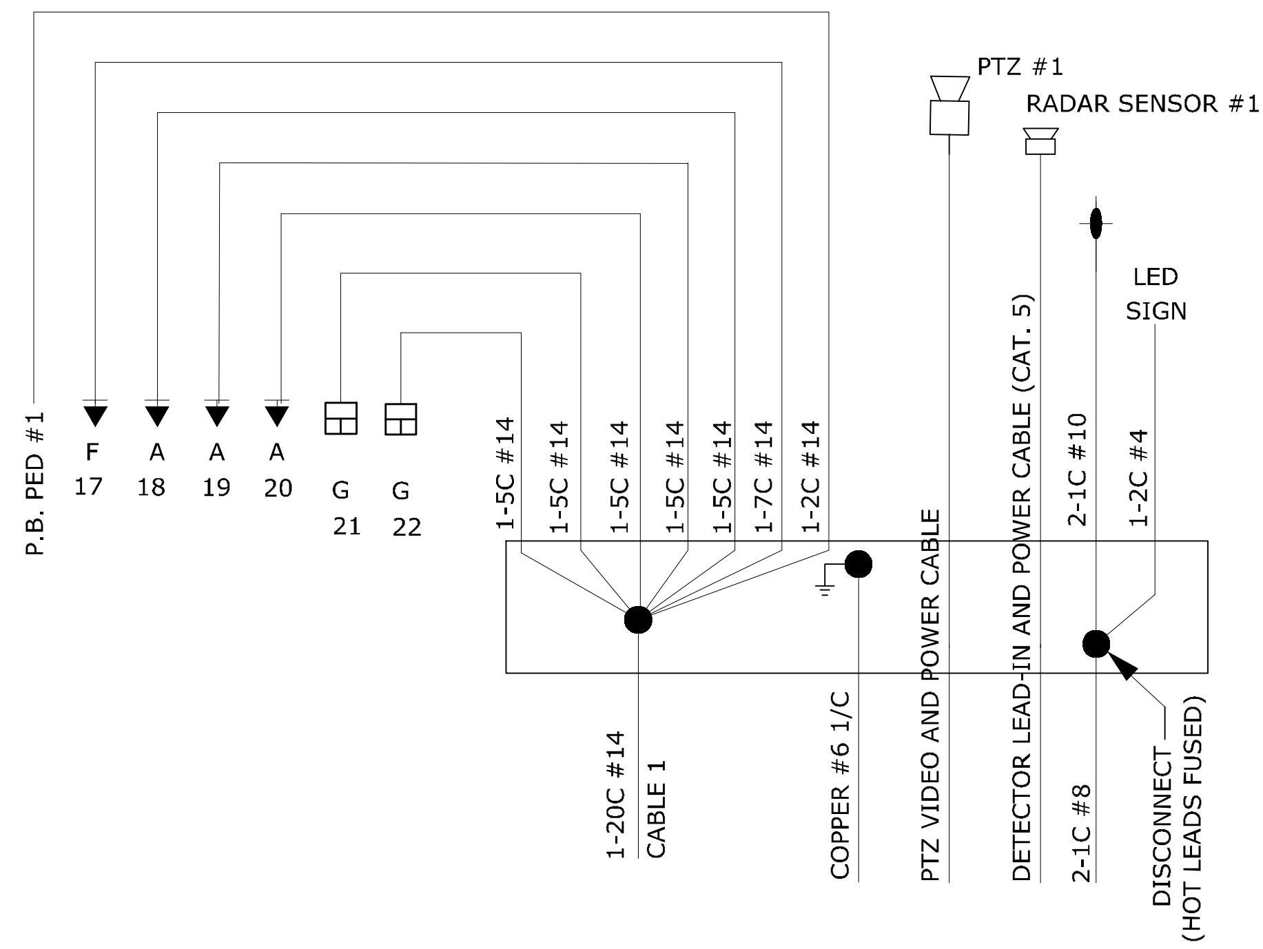
POLE #1
