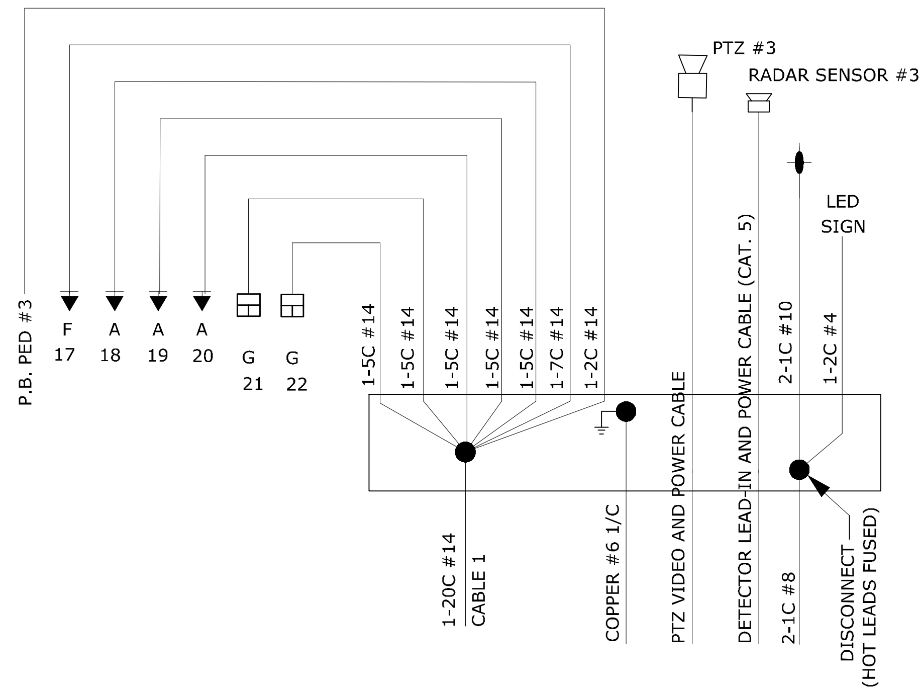
POLE #3
